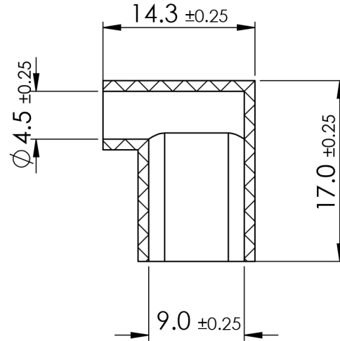
SECTION Y-Y
